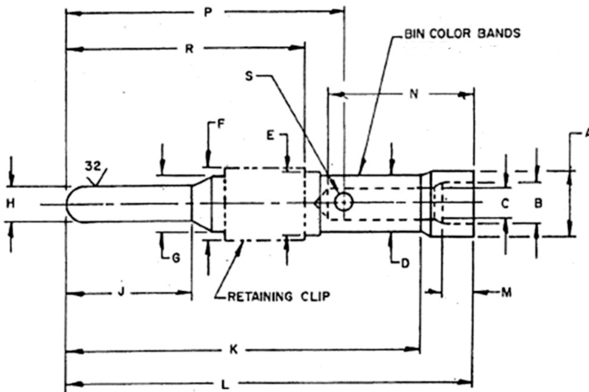
FIGURE 1- AS39029/34 PIN CONTACT
