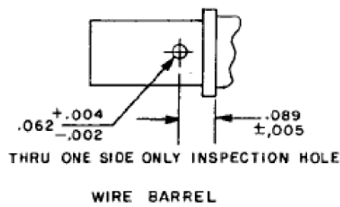
FIGURE 2 – WIRE BARREL (BORE BARREL CRIMP DEPTH)
