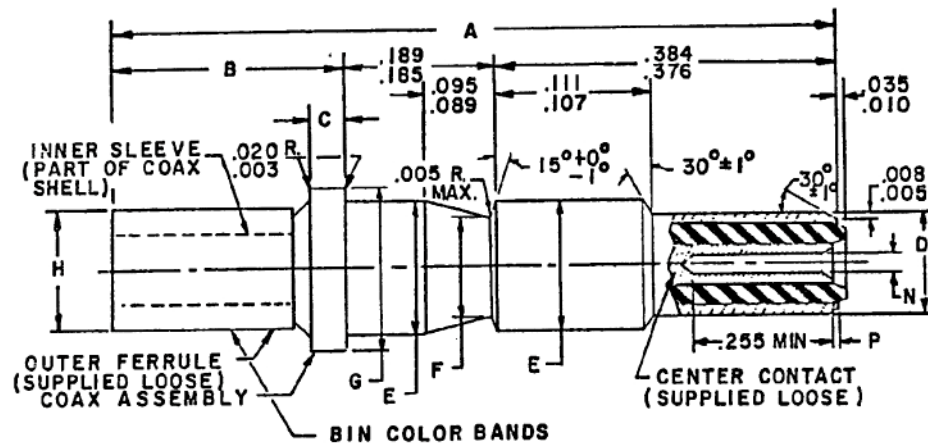
FIGURE 1 – CONNECTOR CONTACT
