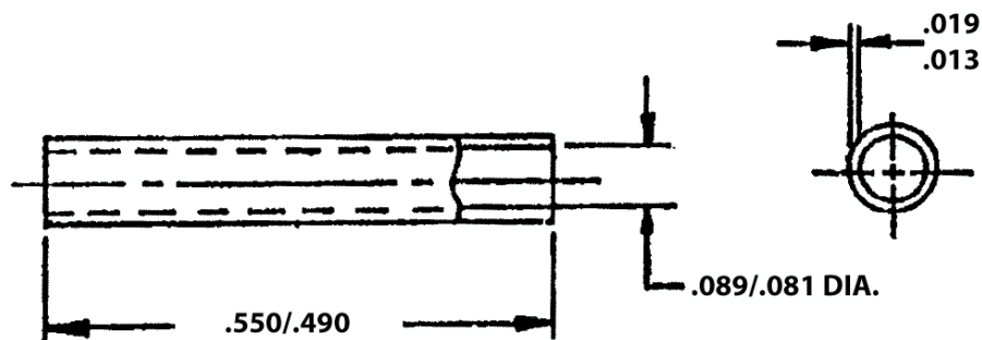
FIGURE 3 - SLEEVE, SEALING, COAXIAL CABLE
