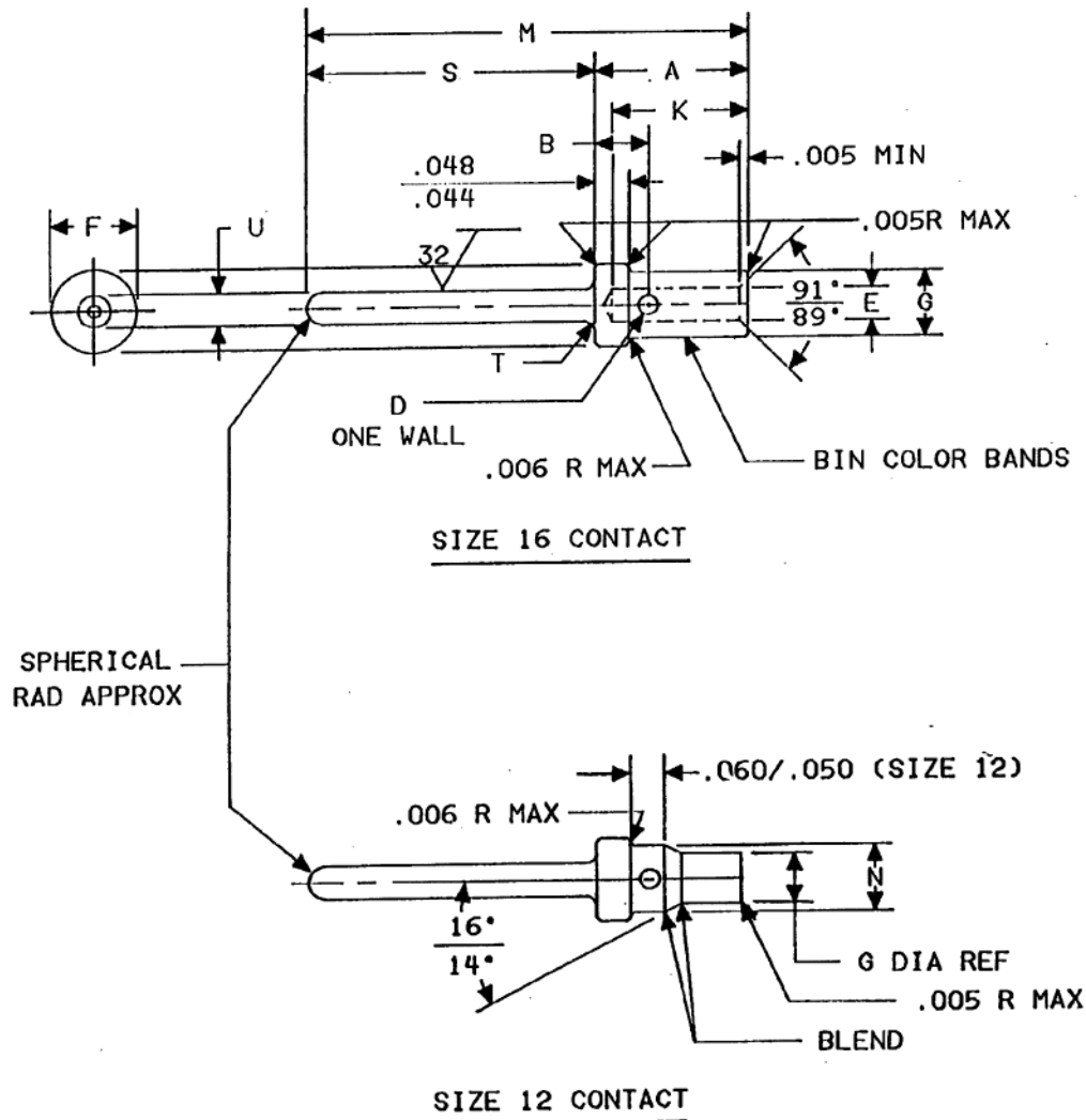
FIGURE 1 - PIN CONTACTS
