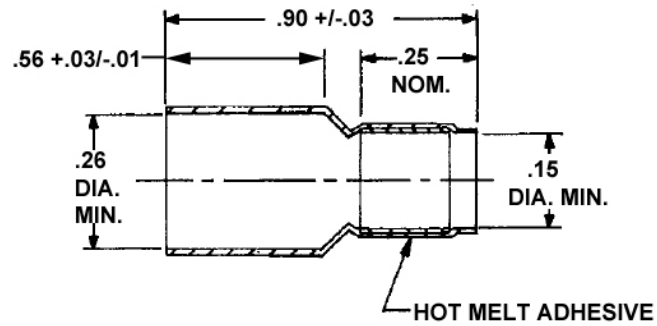
FIGURE 4 - HEAT SHRINK BOOT
