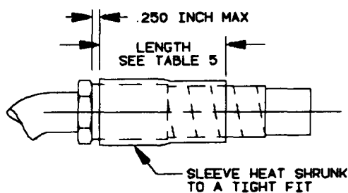
FIGURE 2 - HEAT SHRINKABLE SLEEVES REQUIRED FOR COIL AND TUBULAR ABRASION SLEEVES /6/ AND /7/
