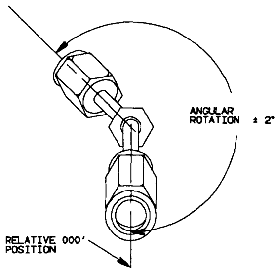
FIGURE 3 - HOSE ASSEMBLY END VIEW
