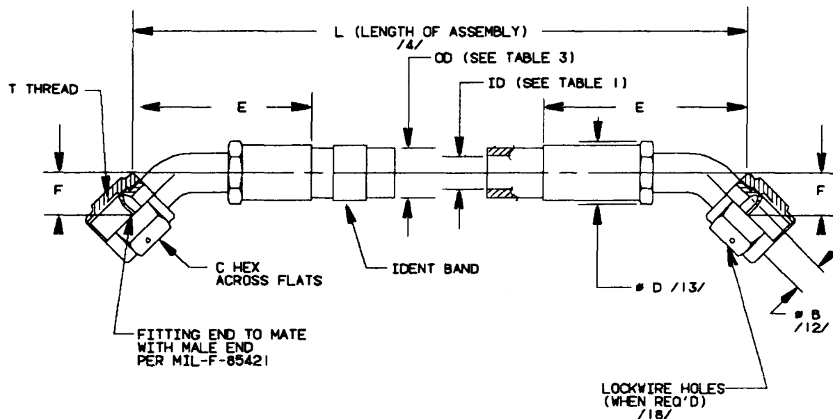
FIGURE 1 - HOSE ASSEMBLY
