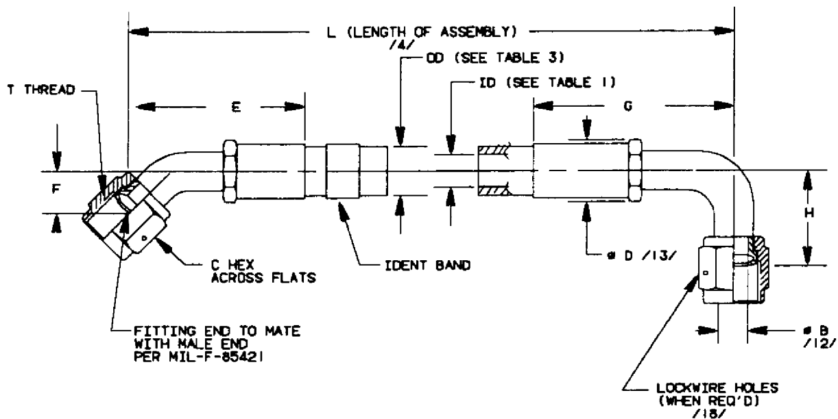
FIGURE 1 - HOSE ASSEMBLY
