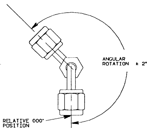
FIGURE 3 - HOSE ASSEMBLY END VIEW
