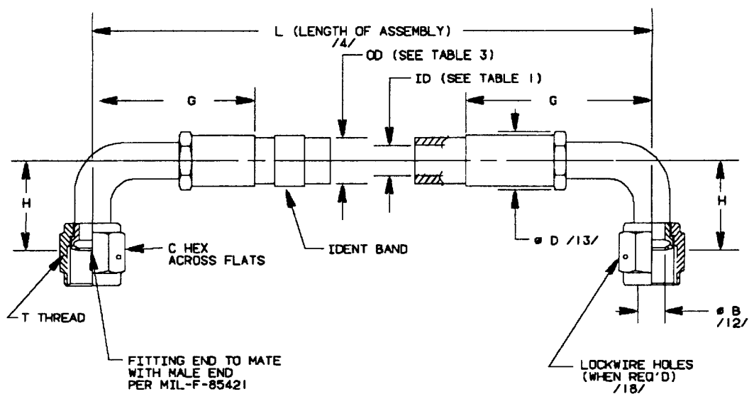
FIGURE 1 - HOSE ASSEMBLY
