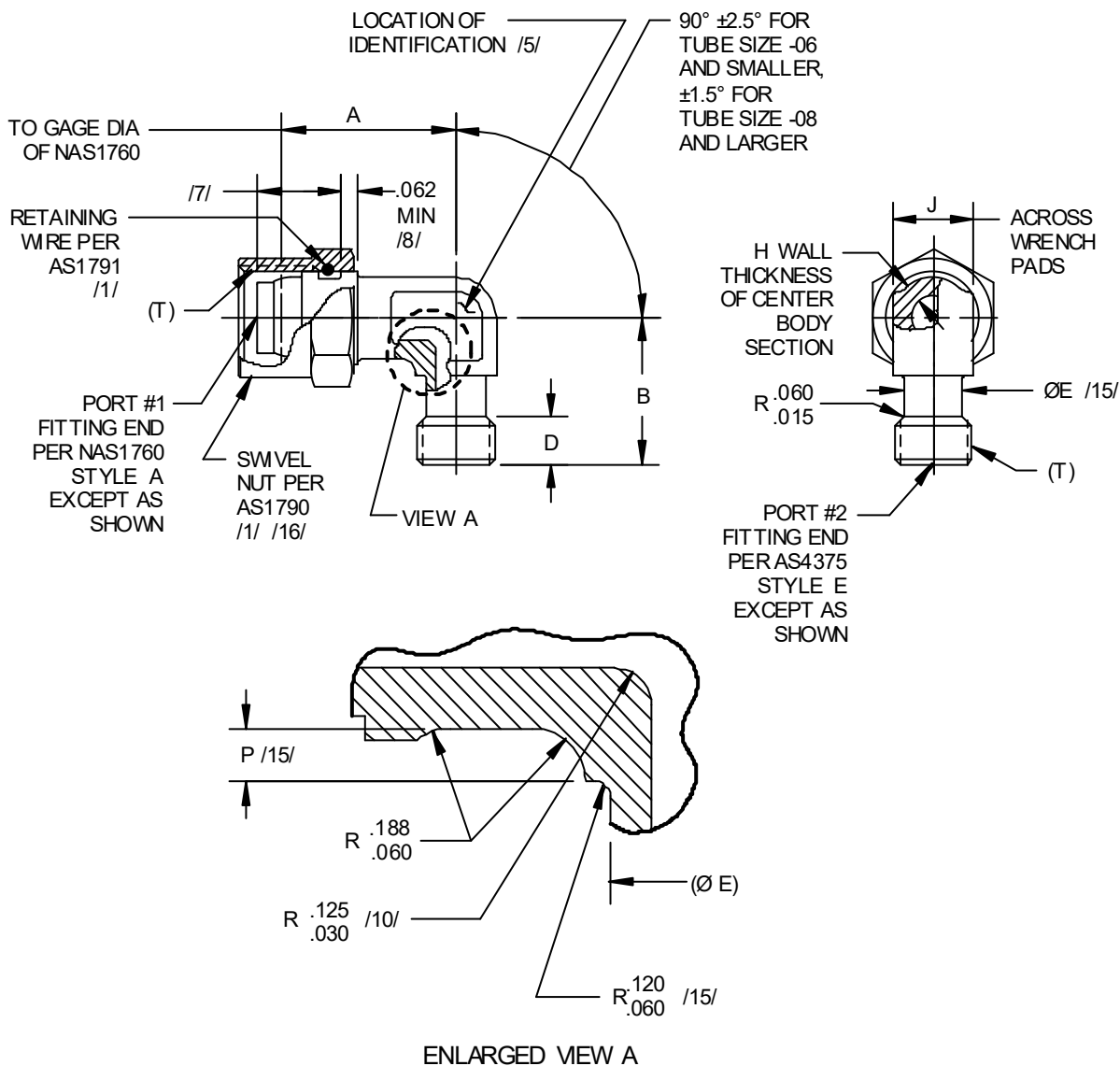
FIGURE 1 - FITTING ASSY, ELBOW, REDUCER, 90°, SWIVEL, REDUCED BODY, FLARELESS
