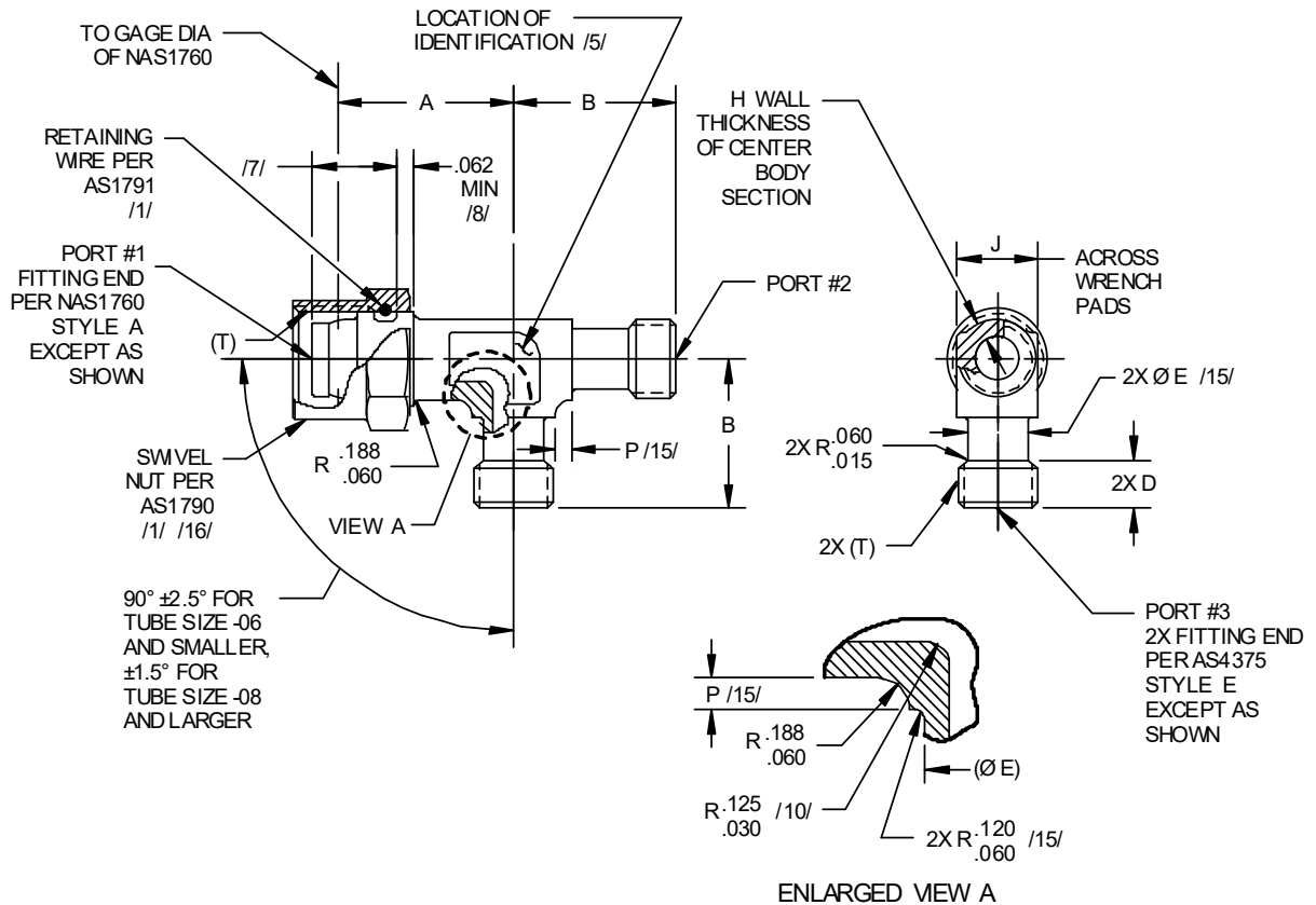
FIGURE 1 - FITTING ASSY, TEE, REDUCER, SWIVEL ON RUN, REDUCED BODY, FLARELESS
