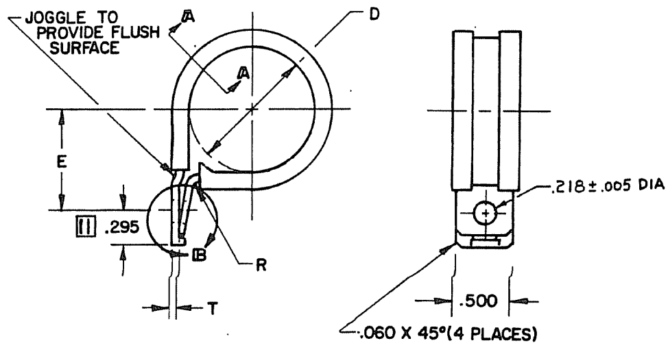
FIGURE 1-CLAMP DESIGN AND DIMENSIONS
