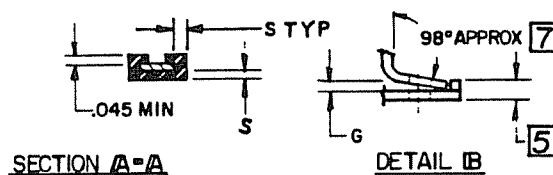
FIG 3 ACCEPTABLE WEDGE CONFIGURATIONS [10]
