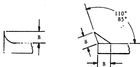
FIG 3 ACCEPTABLE WEDGE CONFIGURATIONS [10]
