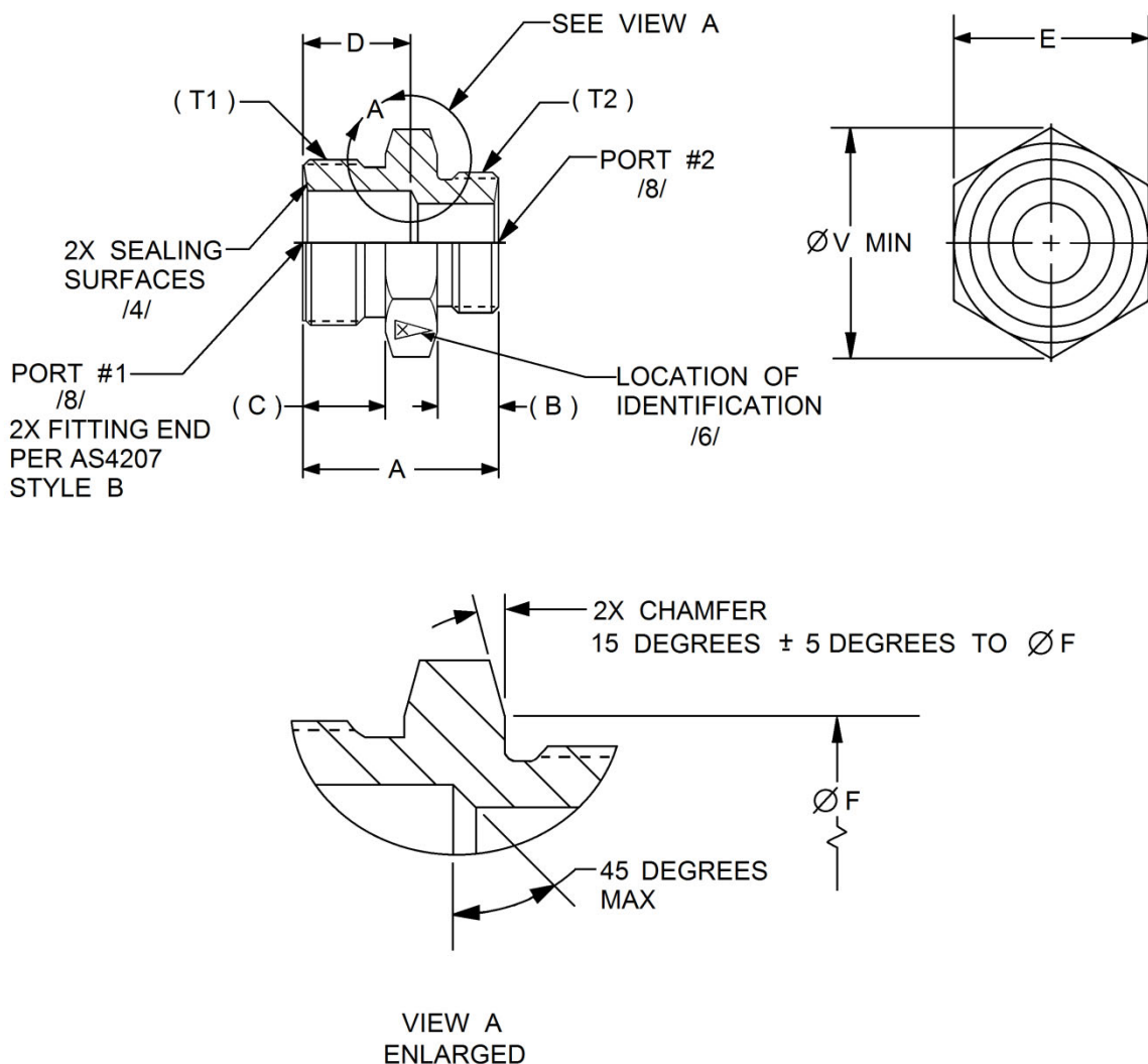
FIGURE 1 - FITTING, UNION, REDUCER
