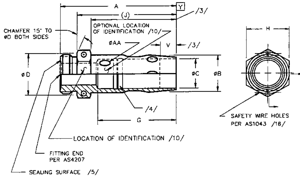
FIGURE 1 - FITTING, BEAM SEAL, EXTERNAL THREAD, EXTERNAL SWAGE TUBE END
