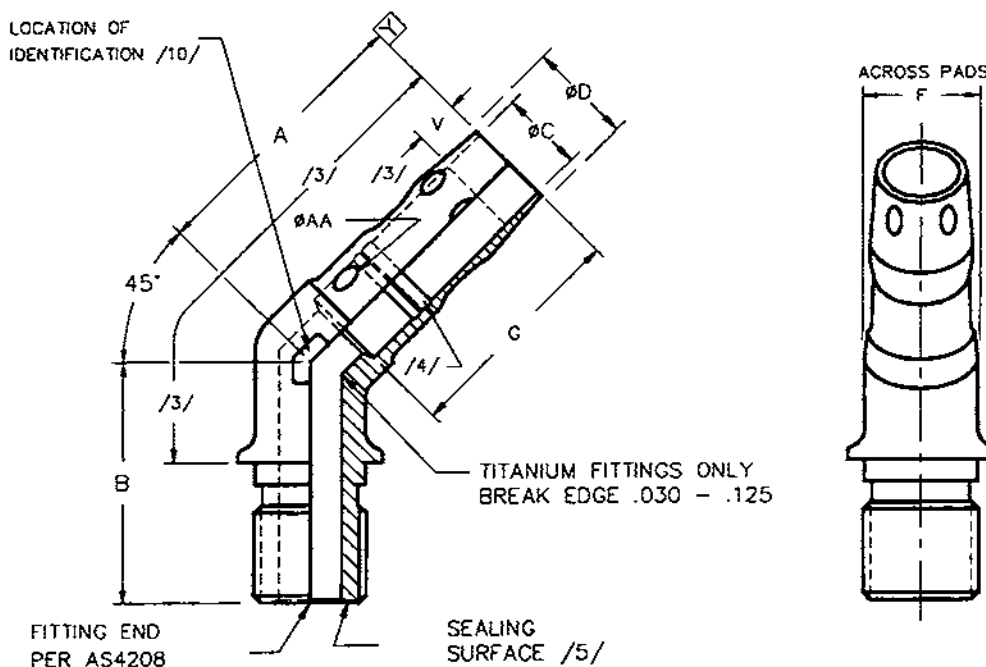
FIGURE 1 - ELBOW, 45°, BEAM SEAL, BULKHEAD
