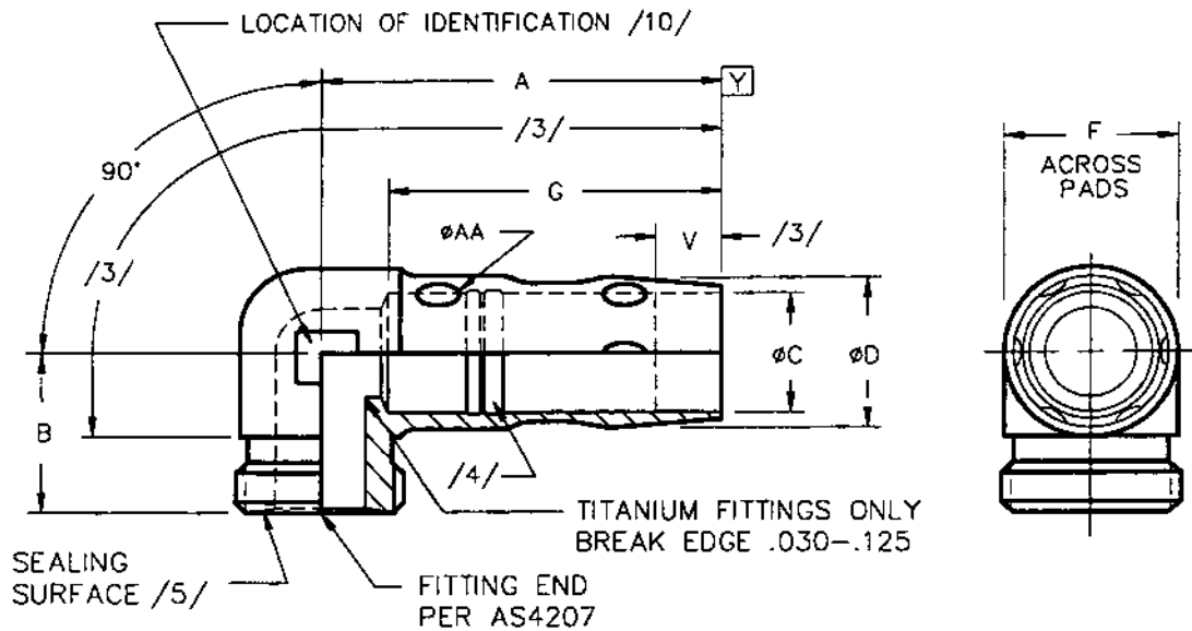
FIGURE 1 - ELBOW, 90°, BEAM SEAL, EXTERNAL THREAD
