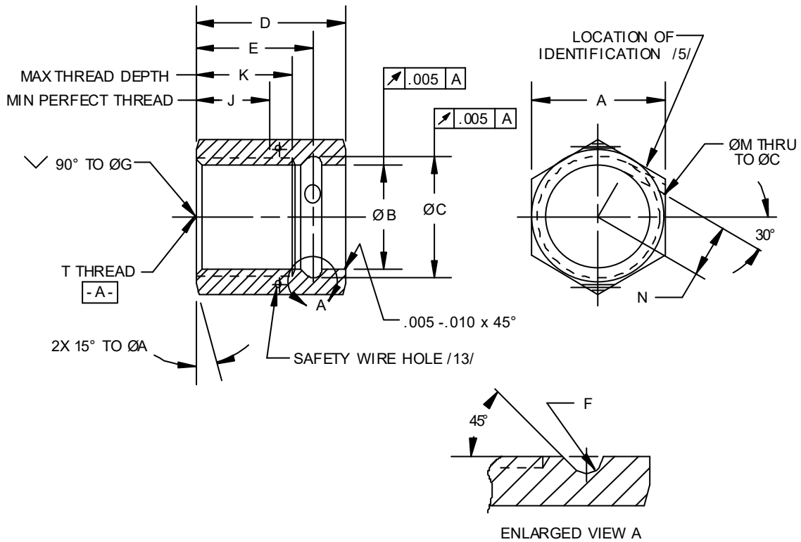
FIGURE 1 - SWIVEL NUT
