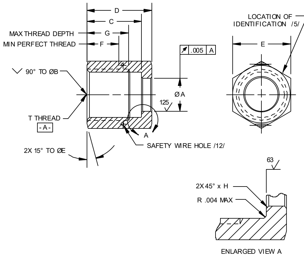
FIGURE 1 - NUT, COUPLING
