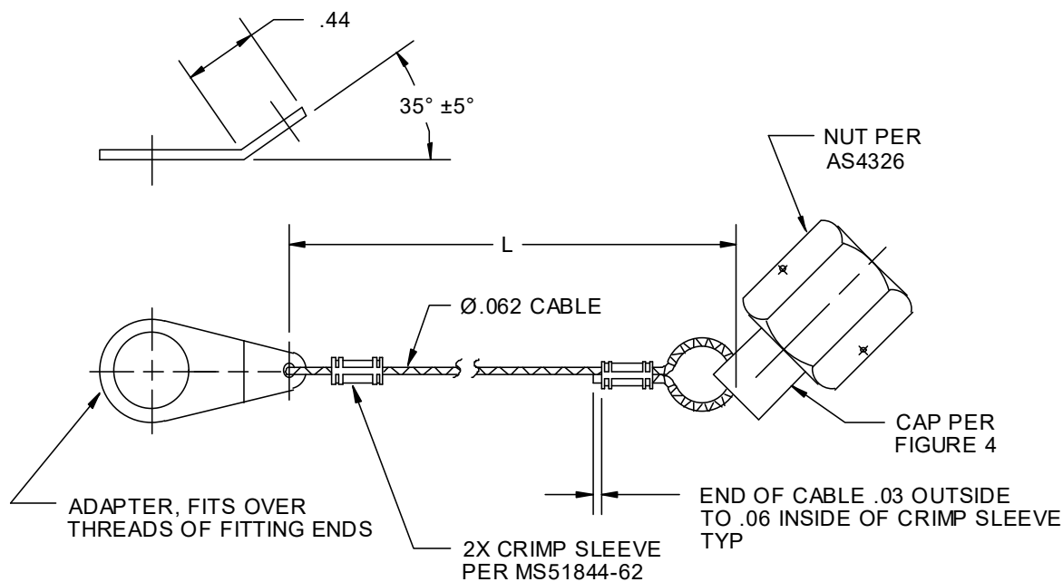
FIGURE 3 - CAP ASSEMBLY - ALTERNATE /7/
