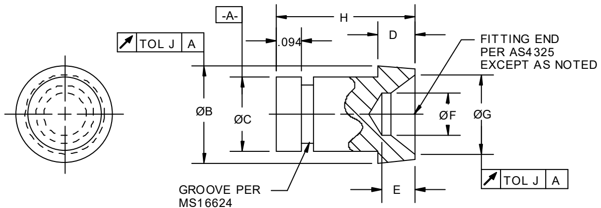
FIGURE 2 - CAP DETAIL - BASIC
