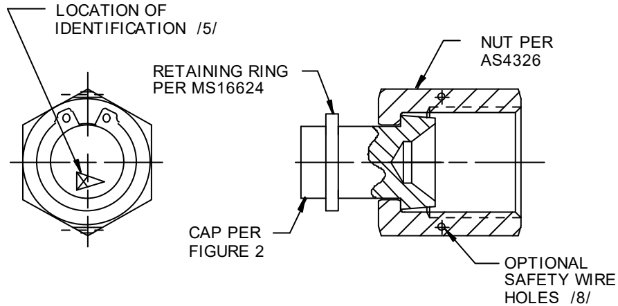
FIGURE 1 - CAP ASSEMBLY - BASIC
