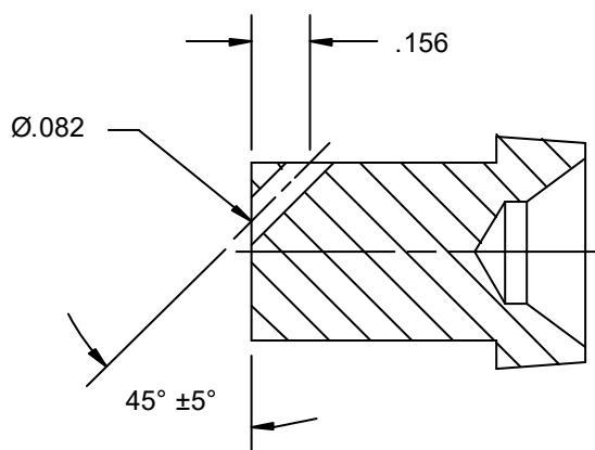
FIGURE 4 - CAP DETAIL - ALTERNATE - SAME AS FIGURE 2, EXCEPT AS SHOWN /7/
