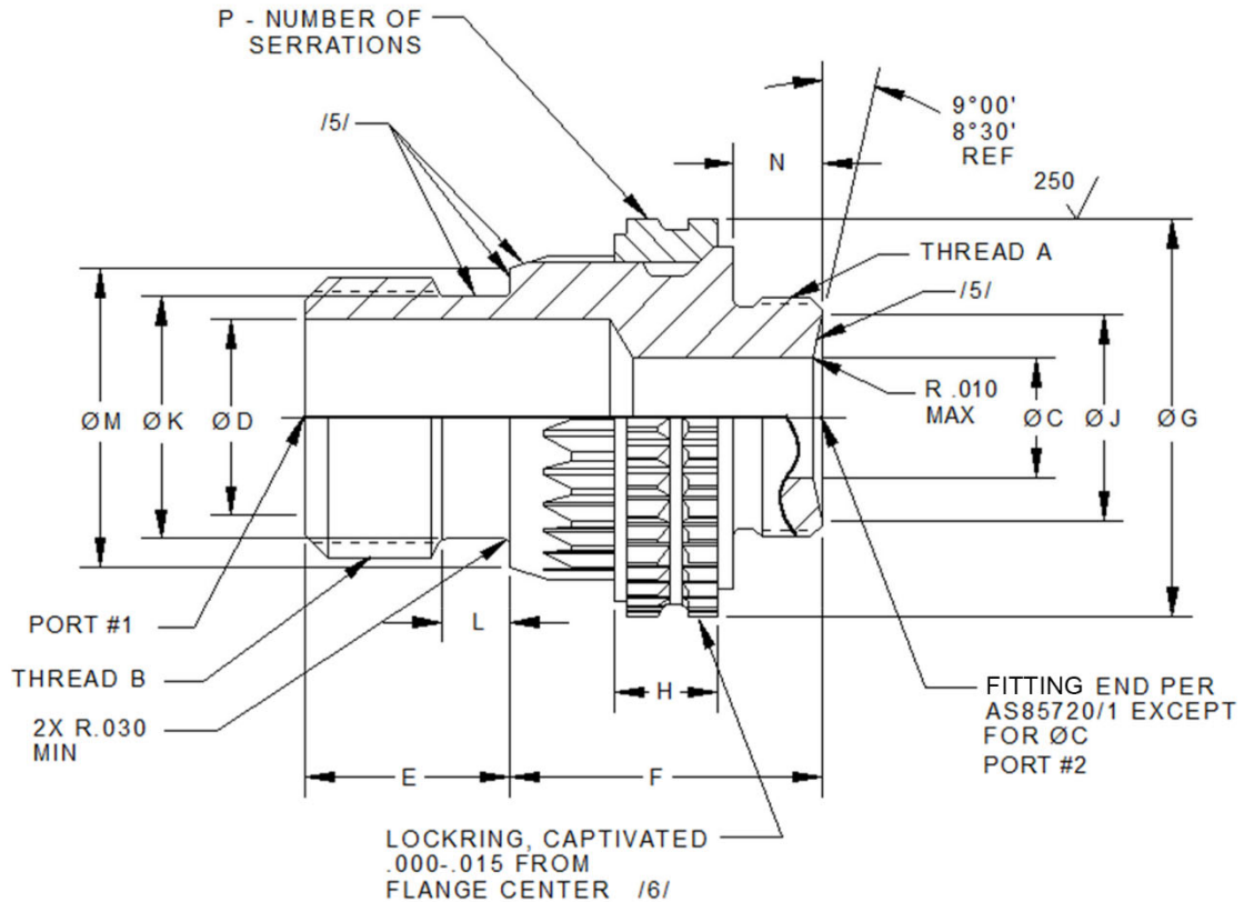
FIGURE 1 - ADAPTER, ASSEMBLY /17/
