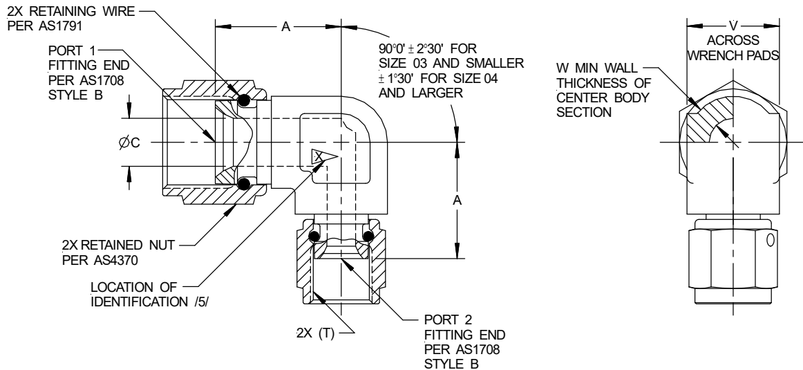
FIGURE 1 - FITTING ASSEMBLY, ELBOW 90°
