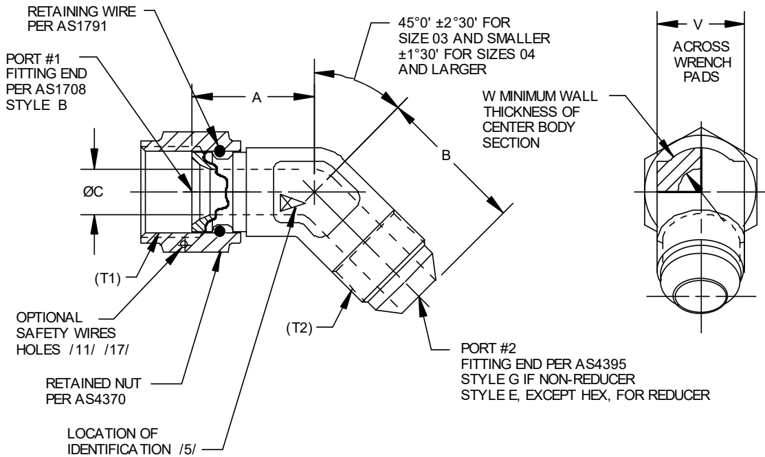
FIGURE 1 - FITTING ASSEMBLY, ELBOW 45°
