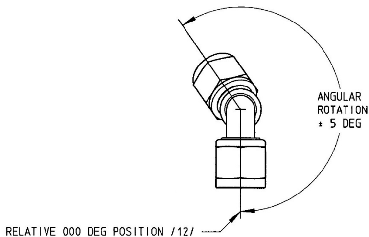
FIGURE 2 - FITTING ANGULAR ORIENTATION
