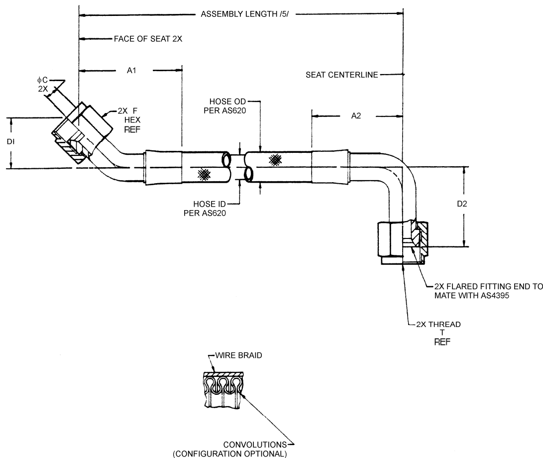
FIGURE 1 - HOSE ASSEMBLY
