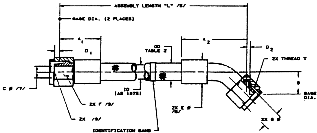
FIGURE 1 - HOSE ASSEMBLY, STRAIGHT TO 45° ELBOW
