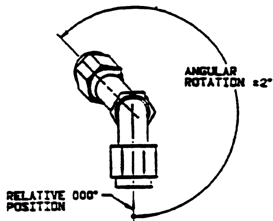
FIGURE 2 - ELBOWS ORIENTATION
