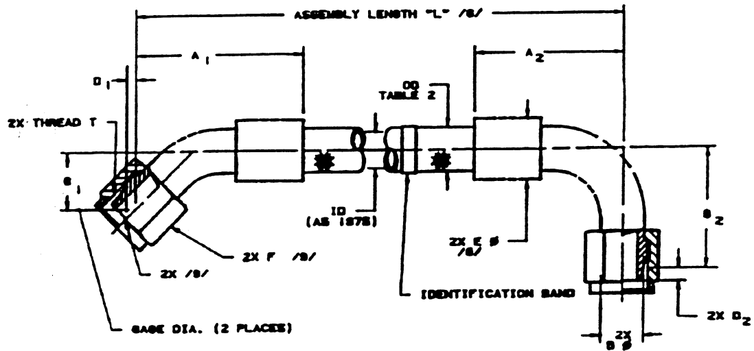
FIGURE 1 - HOSE ASSEMBLY, 45° ELBOW TO 90° ELBOW
