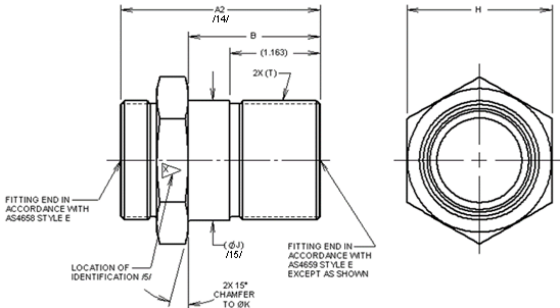
FIGURE 2 - FITTING, UNION, BULKHEAD, EXTENDED LENGTH, SHORT FLARELESS
