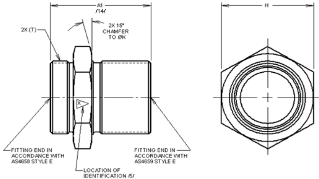
FIGURE 1 - FITTING, UNION, BULKHEAD, STANDARD LENGTH, SHORT FLARELESS
