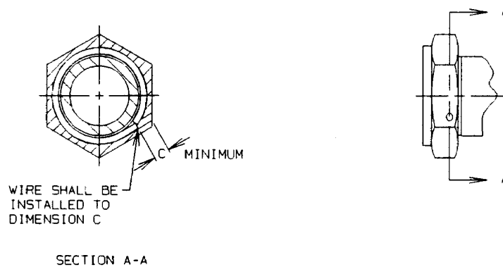
FIGURE 2 - INSTALLATION, RETAINED NUT, AND RETAINING WIRE
