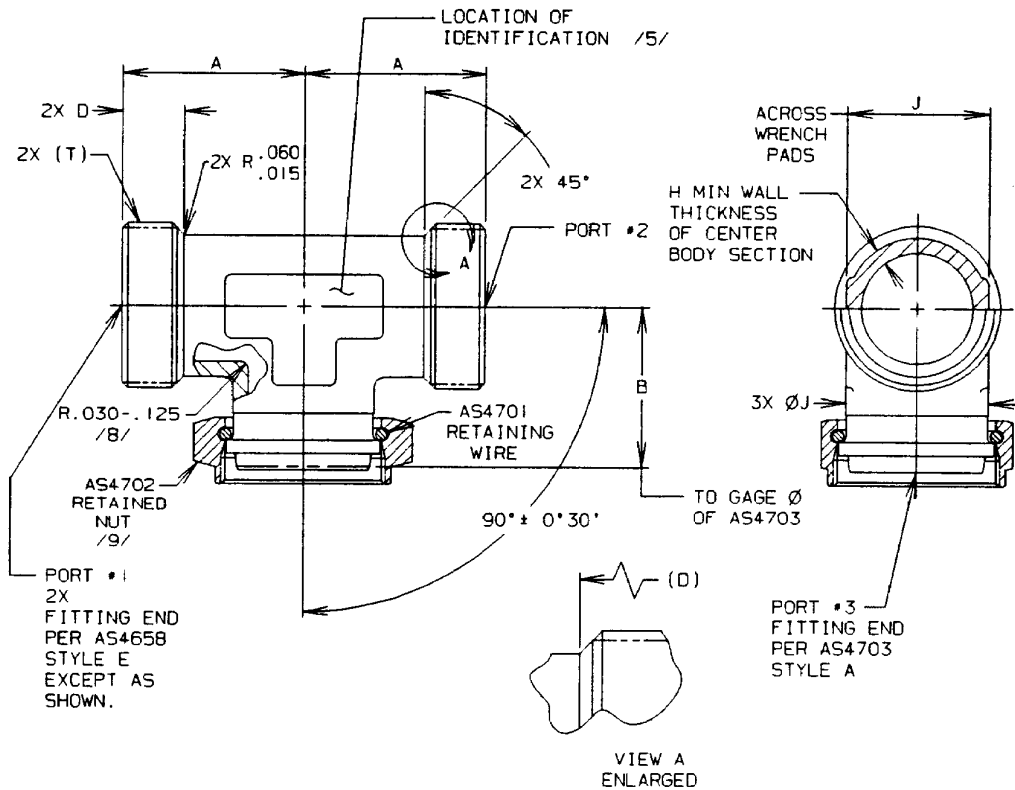
FIGURE 1 - TEE ASSEMBLY
