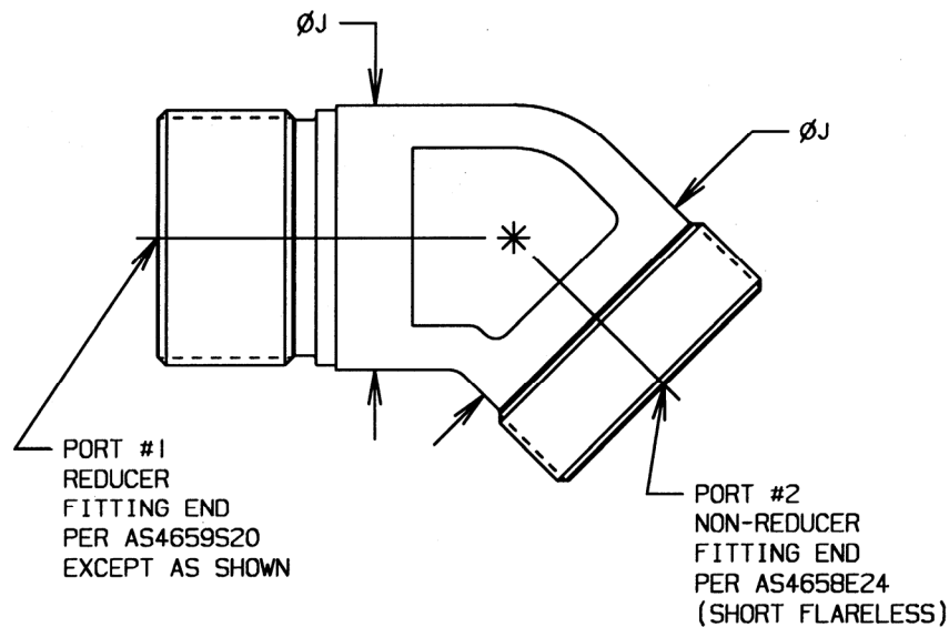
FIGURE 2B - FITTING, ELBOW, 45°, SIZE 20 BULKHEAD REDUCER TO SIZE 24 SHORT END
