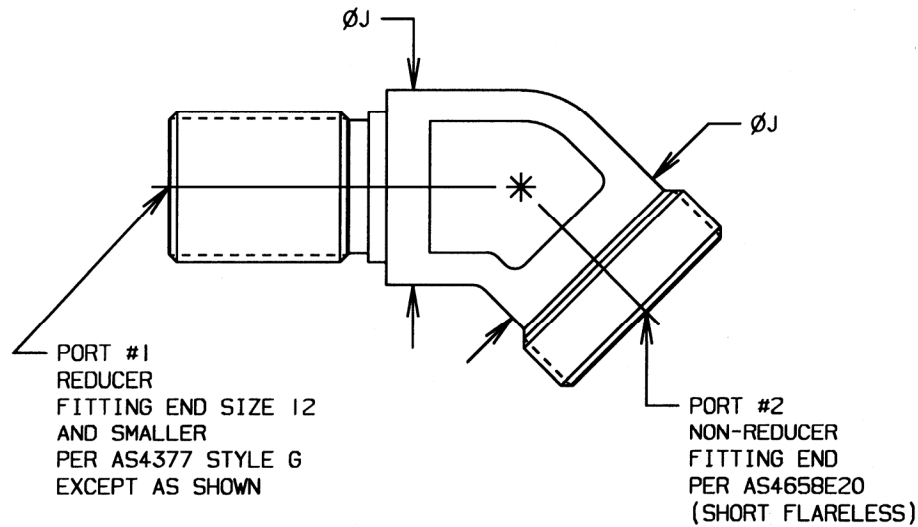
FIGURE 2C - FITTING, ELBOW, 45°, SIZE 12 AND SMALLER BULKHEAD REDUCER TO SIZE 20 SHORT END
