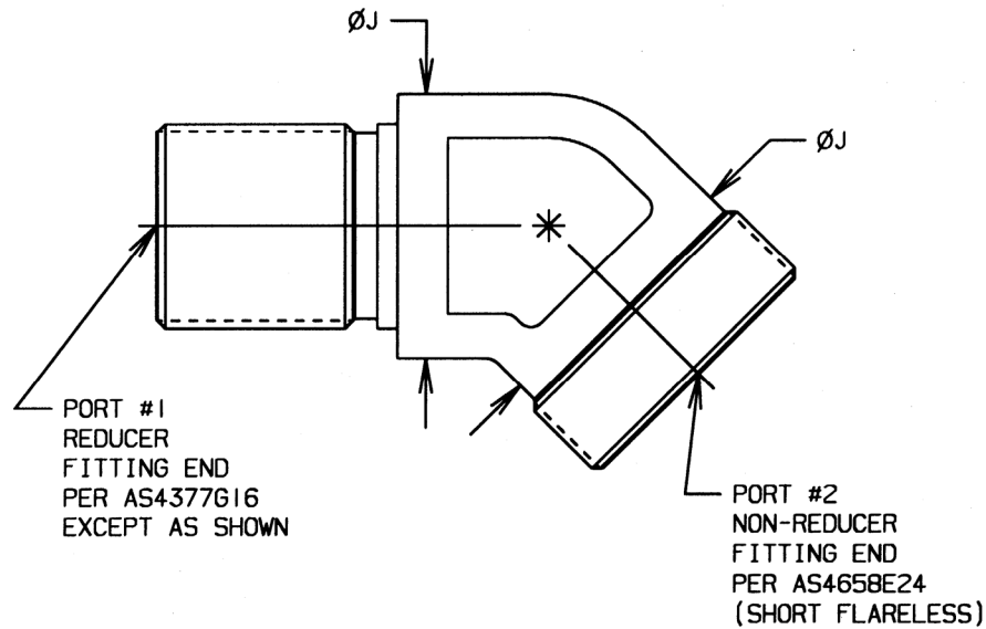
FIGURE 2D - FITTING, ELBOW, 45°, SIZE 16 BULKHEAD REDUCER TO SIZE 24 SHORT END
