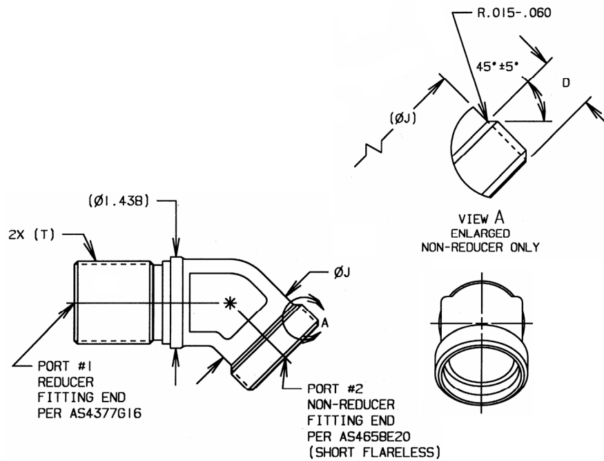
FIGURE 2A - FITTING, ELBOW, 45°, SIZE 16 BULKHEAD REDUCER TO SIZE 20 SHORT END
