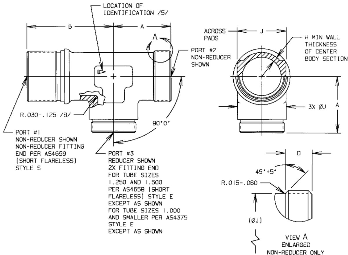
FIGURE 1 - FITTING, TEE, REDUCER
