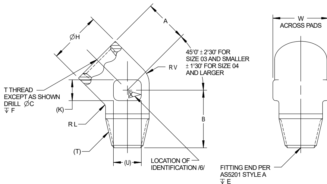
FIGURE 1 – FITTING, ELBOW, 45°, PIPE, INTERNAL AND EXTERNAL THREAD
