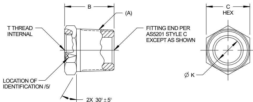
FIGURE 1 – FITTING, BUSHING, PIPE, INTERNAL AND EXTERNAL THREAD
