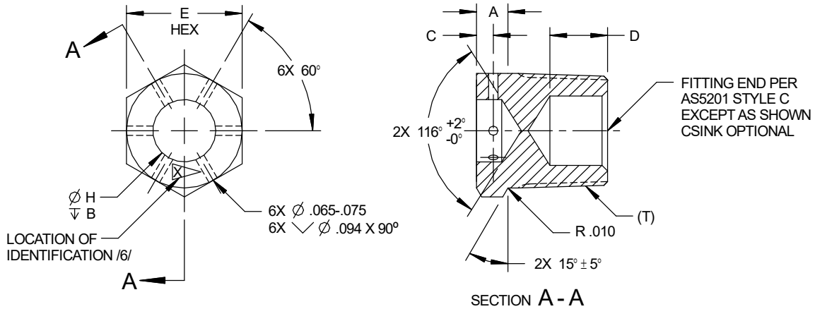
FIGURE 1 - PLUG, PIPE, EXTERNAL THREAD, HEX HEAD
