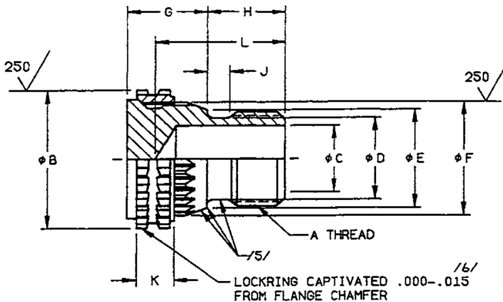
FIGURE 1 - PLUG, ASSEMBLY
