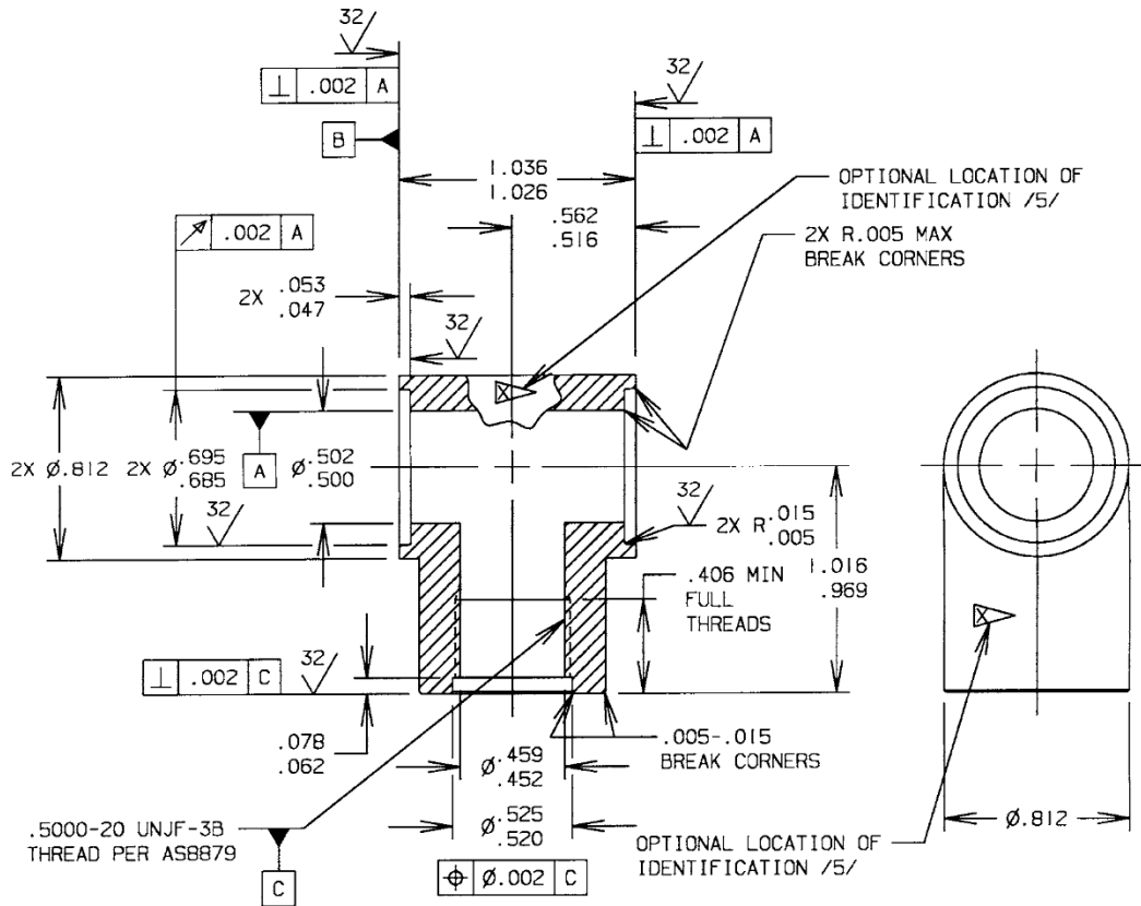
FIGURE 1 - FITTING, TEE /13/
