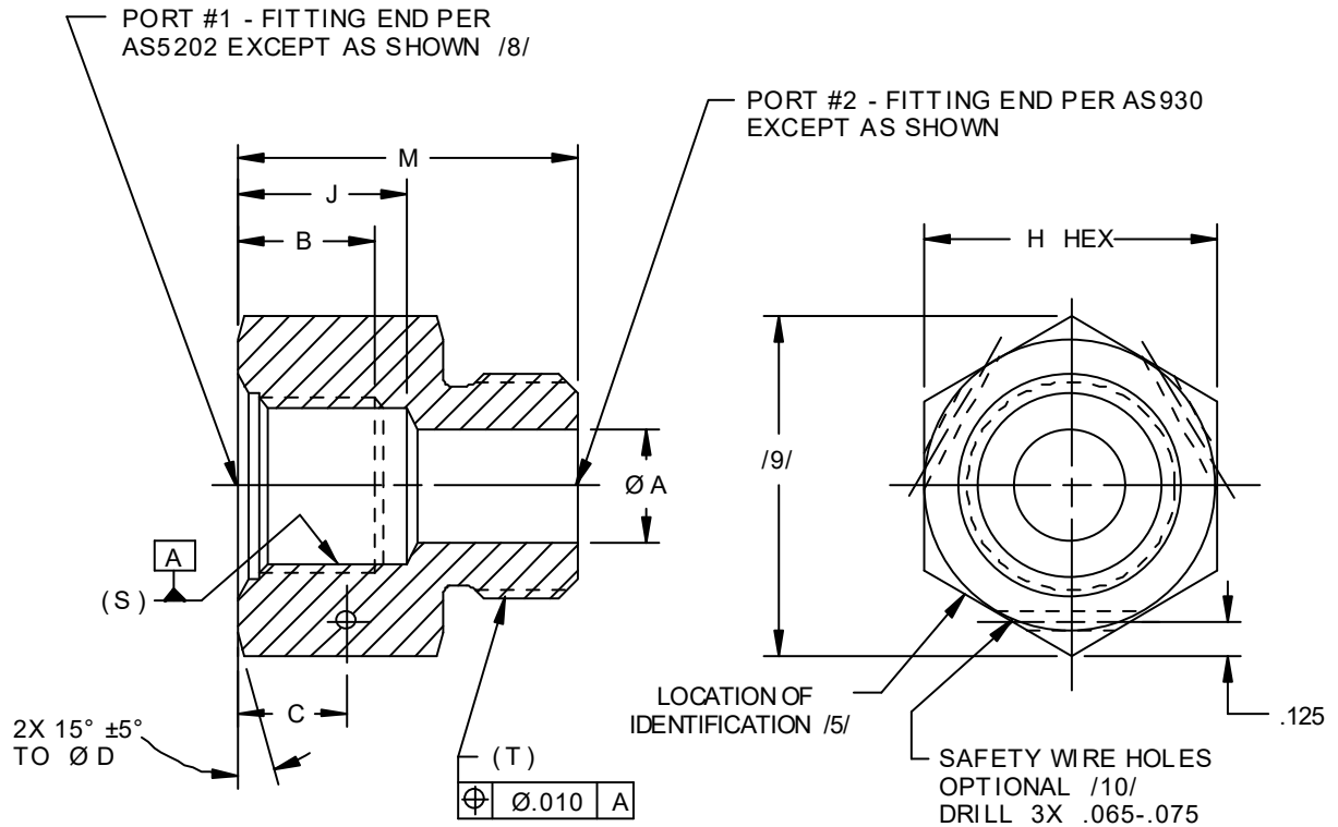
FIGURE 1 - FITTING ADAPTER
