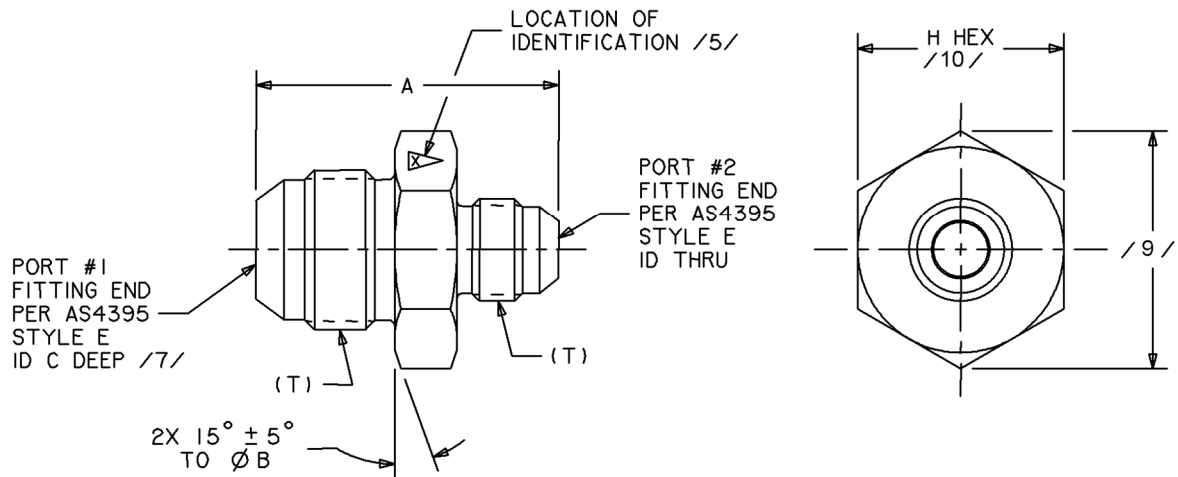
FIGURE 1 - FITTING, UNION AND REDUCER
