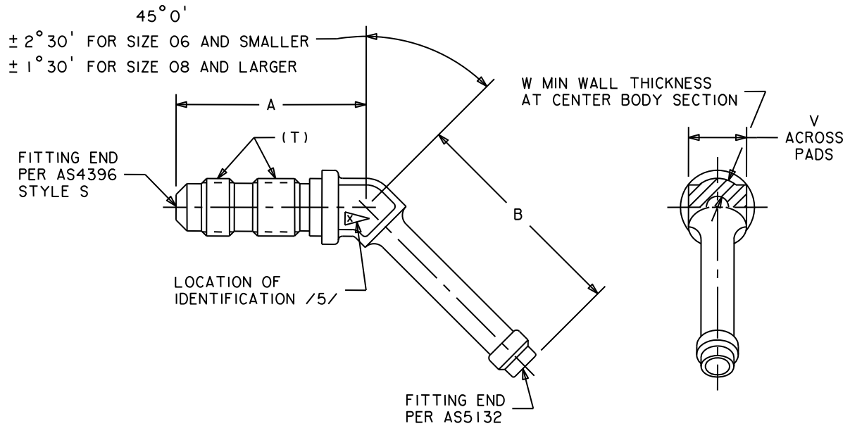
FIGURE 1 – FITTING, ELBOW, 45°
