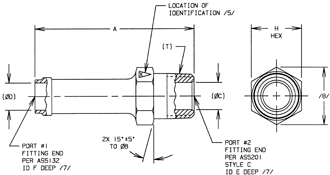
FIGURE 1 - FITTING, ADAPTER
