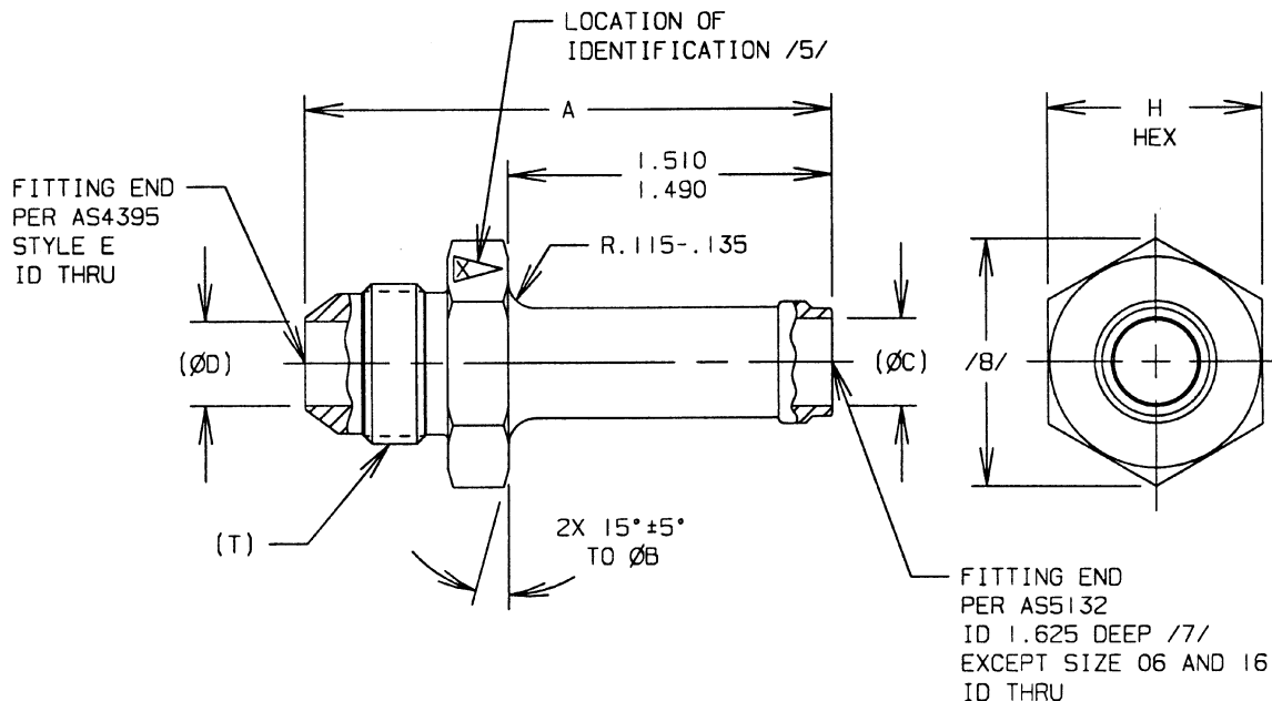
FIGURE 1 - FITTING, ADAPTER
