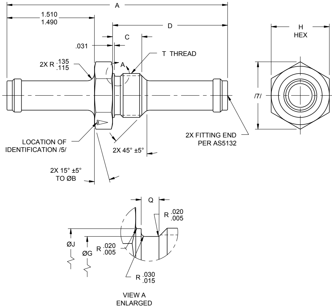
FIGURE 1 - FITTING, ADAPTER
