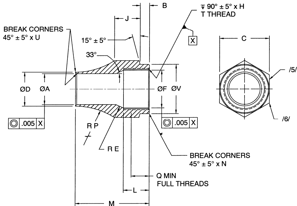
FIGURE 1 - NUT
