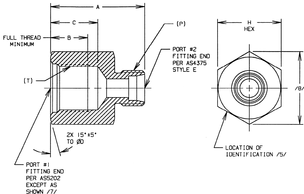
FIGURE 1 - FITTING, ADAPTER
