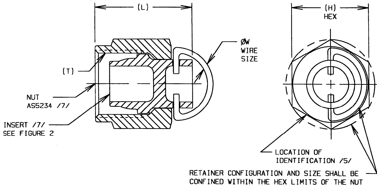
FIGURE 1 - FITTING ASSEMBLY, CAP /16/
