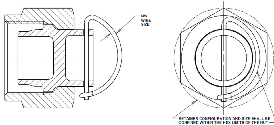
FIGURE 2 - ALTERNATIVE WIRE DESIGN FOR CAP ASSEMBLY /16/
