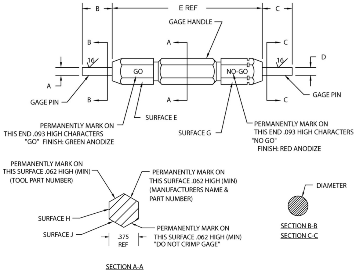
FIGURE 1 - INSPECTION GAGE FOR CRIMP DIES SPECIFIED IN TABLE 1
