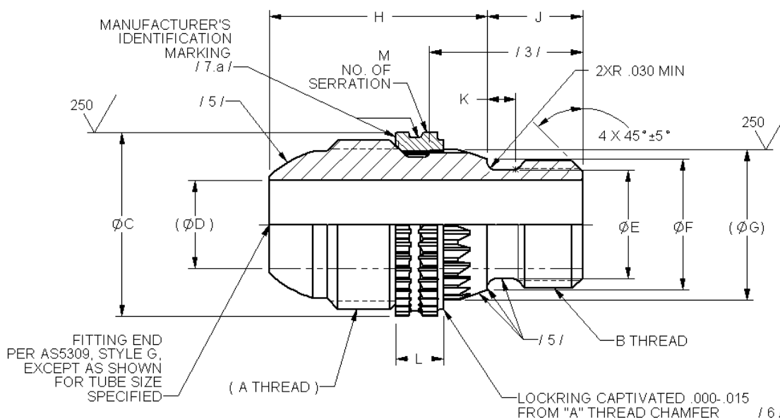
FIGURE 1 - ADAPTER ASSEMBLY
