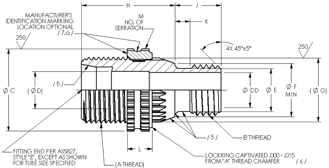
FIGURE 1 - FITTING ASSEMBLY
