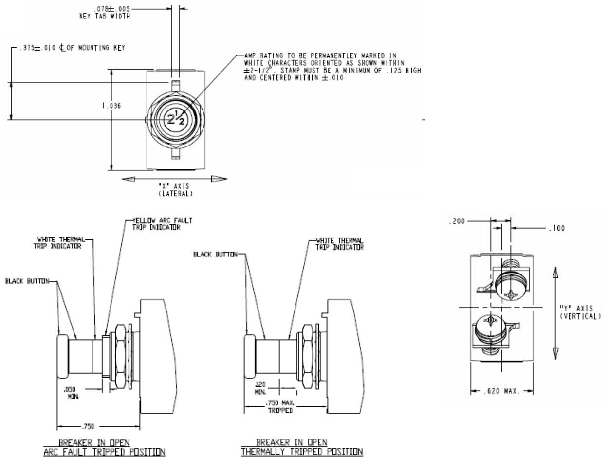
FIGURE 2 - CIRCUIT BREAKER CONFIGURATIONS AND DIMENSIONS (CONTINUED)
