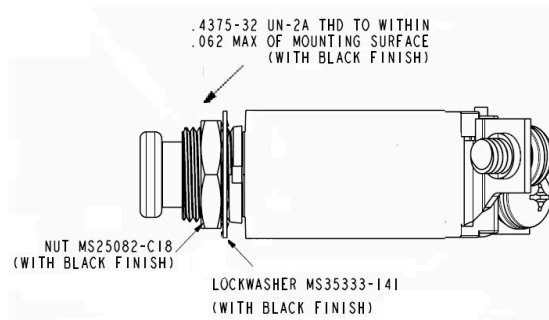
FIGURE 1 - CIRCUIT BREAKER CONFIGURATIONS AND DIMENSIONS (CONT'D)
