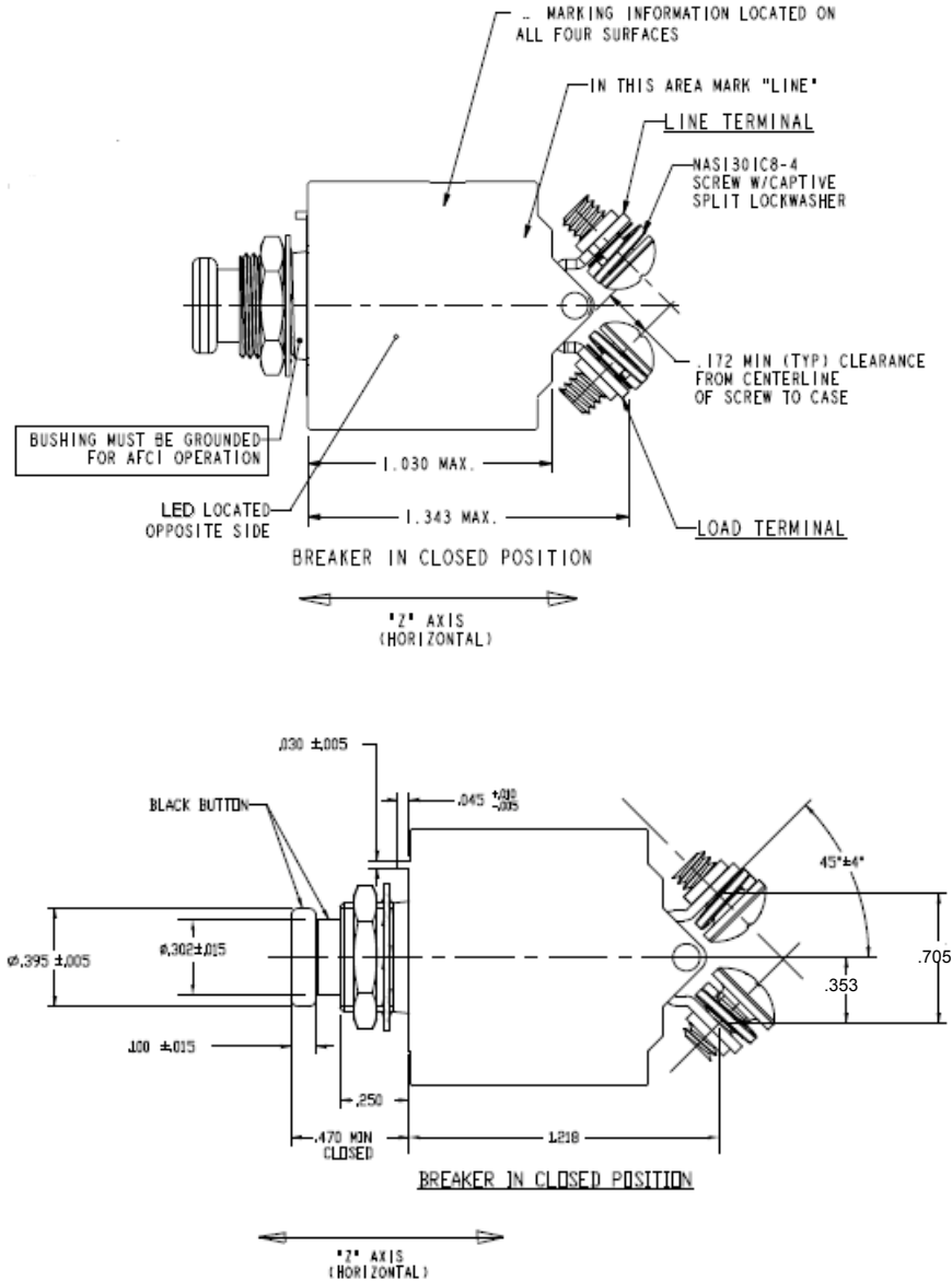
FIGURE 1 - CIRCUIT BREAKER CONFIGURATIONS AND DIMENSIONS
