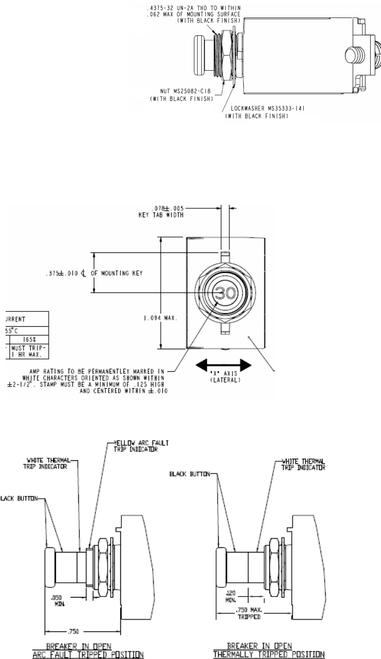
FIGURE 1 - CIRCUIT BREAKER CONFIGURATIONS AND DIMENSIONS (CONT'D)
